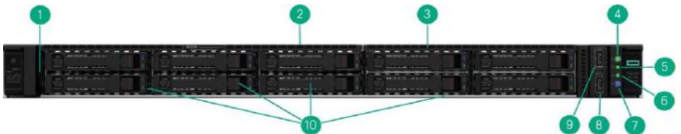
Front View - 8 SFF + optional 2 SFF Drive Bay shown
